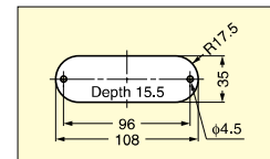
Panel Cut Out Dimensions
