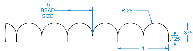
DETAIL A SCALE 1 : 1
