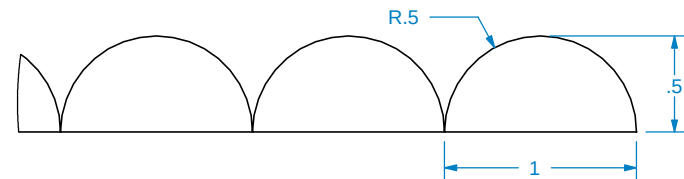
DETAIL A SCALE 1 : 1
