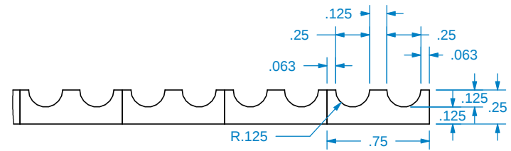
DETAIL A SCALE 1 : 1
